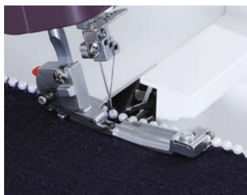
620117496 coverlock™ 4.0 et 3.0 hobbylock™ 2.5
